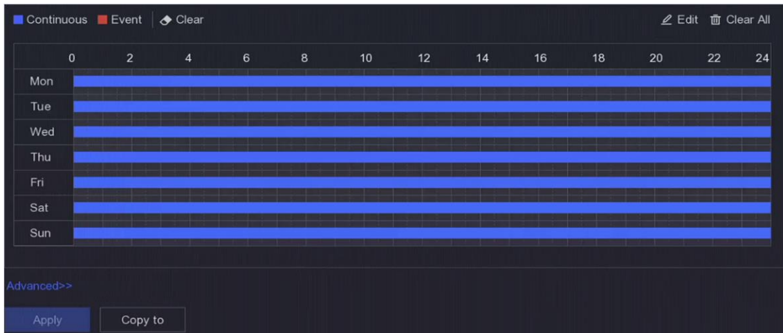
Figure 6-29 Recording Schedule
