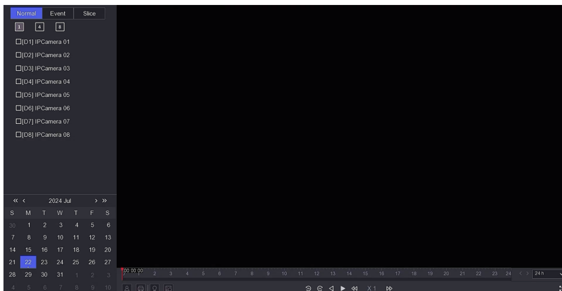
Figure 3-1 Playback
